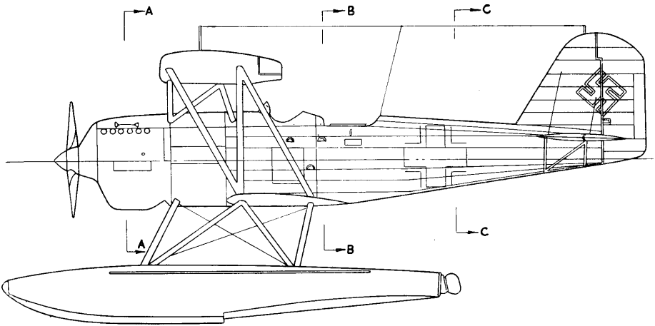
Heinkel He 60 - Typical Fuselage Sections
